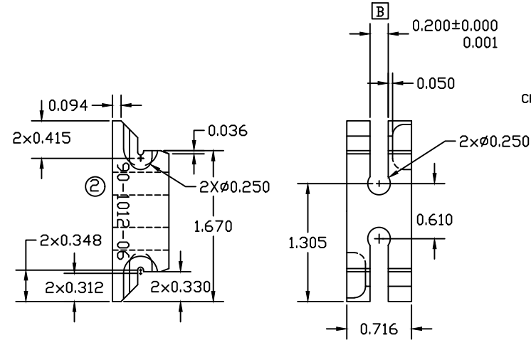
DETAIL A
